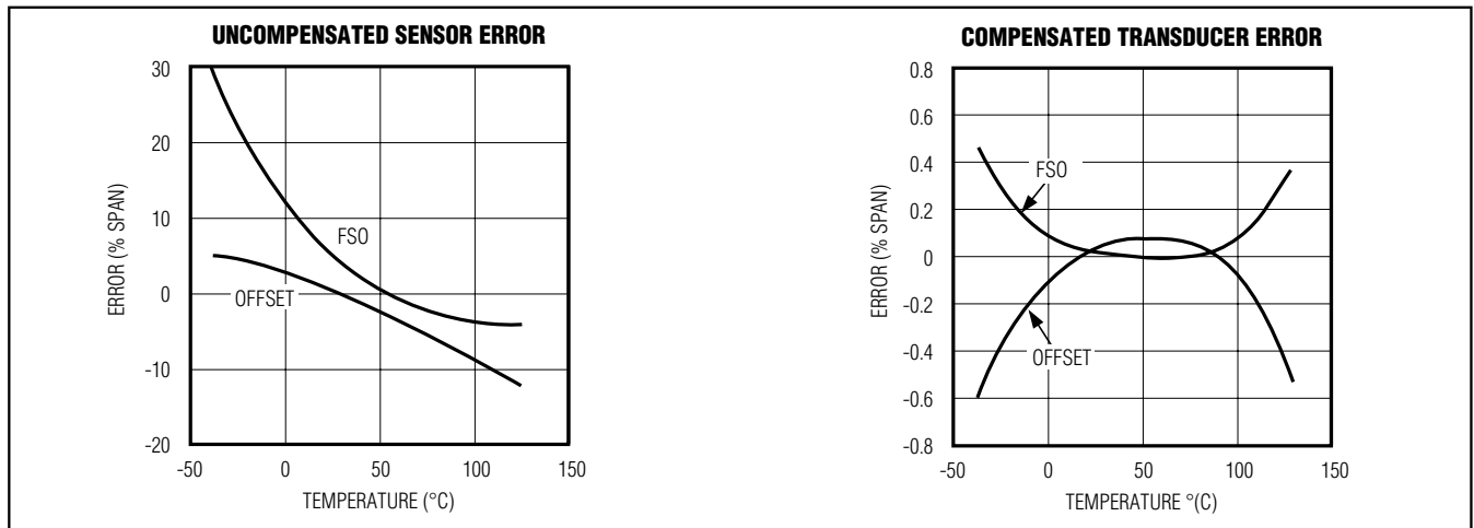
Figure 6. Comparison of an Uncalibrated Sensor and a Temperature-Compensated Transducer
